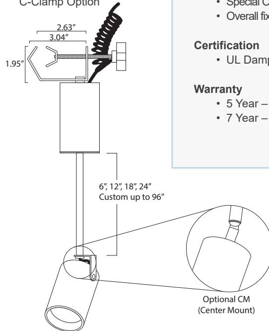
C-Clamp Option
